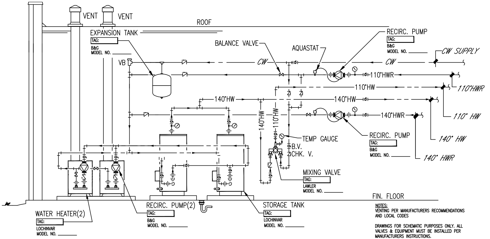
○ TWO HEATERS, TWO TANKS, DUAL TEMPERATURES 2H2T2TPC
